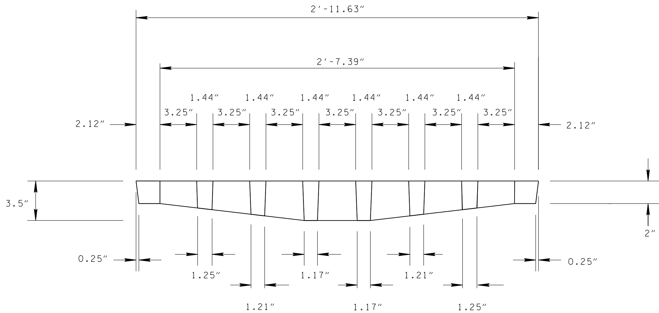
SECTION M-M
